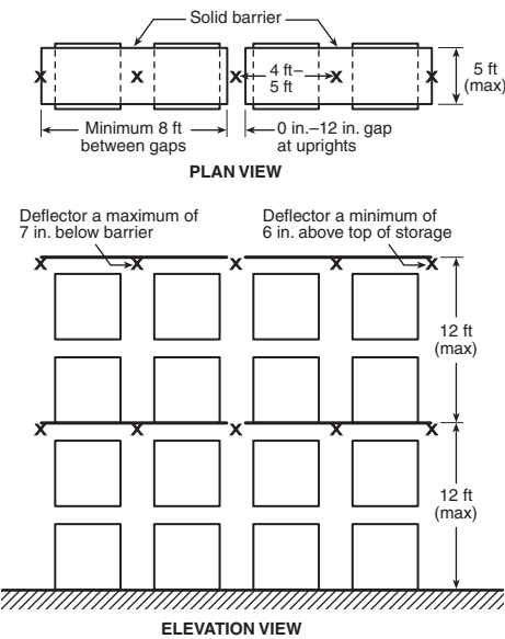
FIGURE 16.6.1.1(a) Single-Row Rack Sprinkler Layout for Design Scheme “A.”
